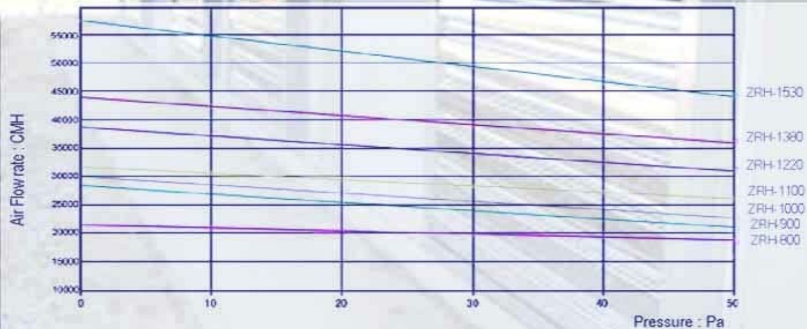
Performance Curve for ZRH Series
